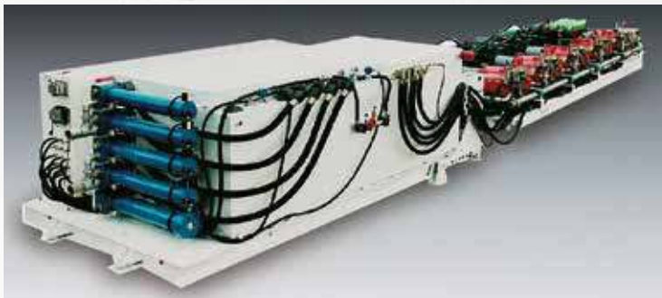
Mobile pump station (pump car) for longwall hydraulics
